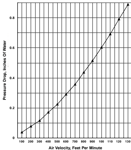
Figure 72D. ULTRA-SAFE™ Pressure Drop Curve
