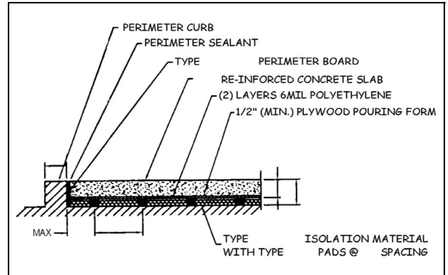
SECTION @ CURB
