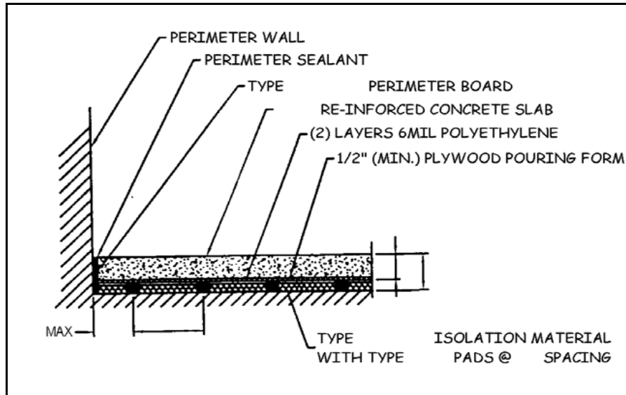
SECTION @ WALL
